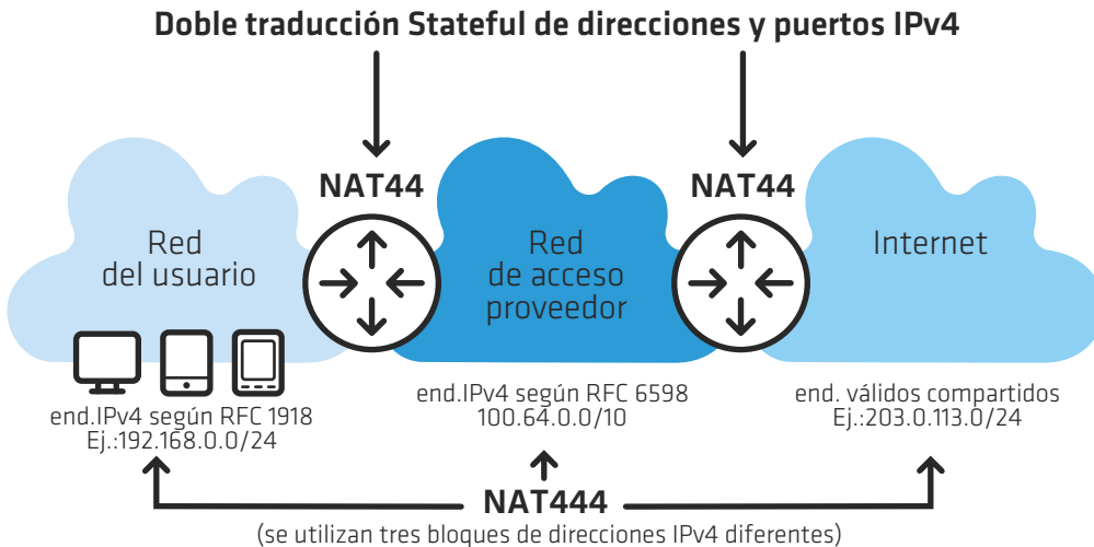
FIGURA 7: NAT444
